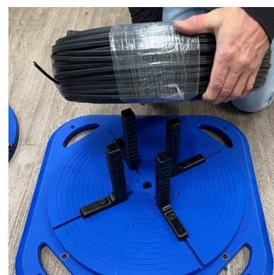
Step 6: Lower cable onto the coil stops.
