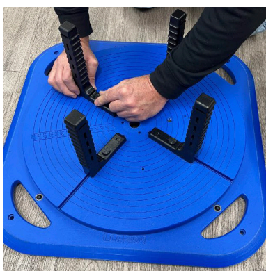
Step 5: Adjust the (4) coil stops to the size of your coil diameter. Loosening the knobs on the coil stops allows you to move the coil stops in and out to the size of your coil. For larger diameter coils, reverse the footing on the coil stops.
