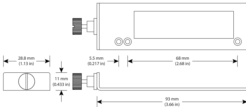
Media Converter Carrier Bracket
