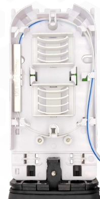
HDPAS-GEL-SA1-S4 PLC Module Installation
