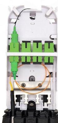
HDPAS-GEL-SA1-P4 SC Adapters with Pigtail Installation
