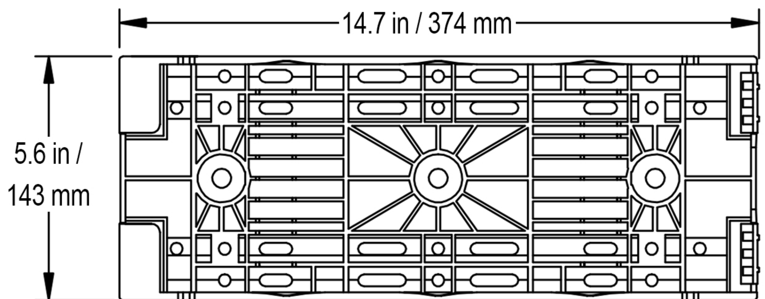
HyperDrop MST Base
