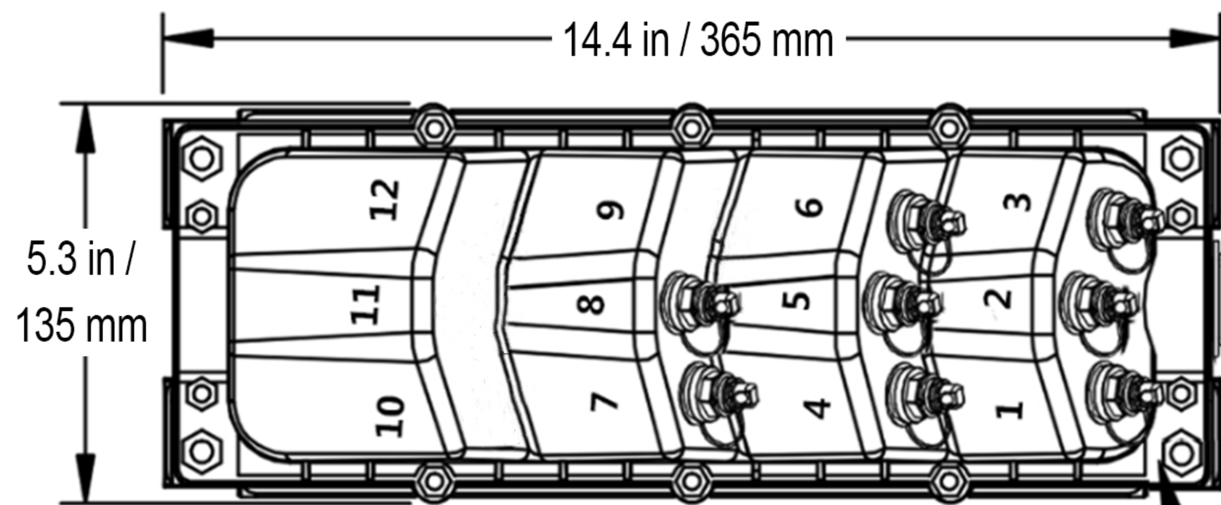
HyperDrop MST-Rapid Deploy Outdoor Terminal
